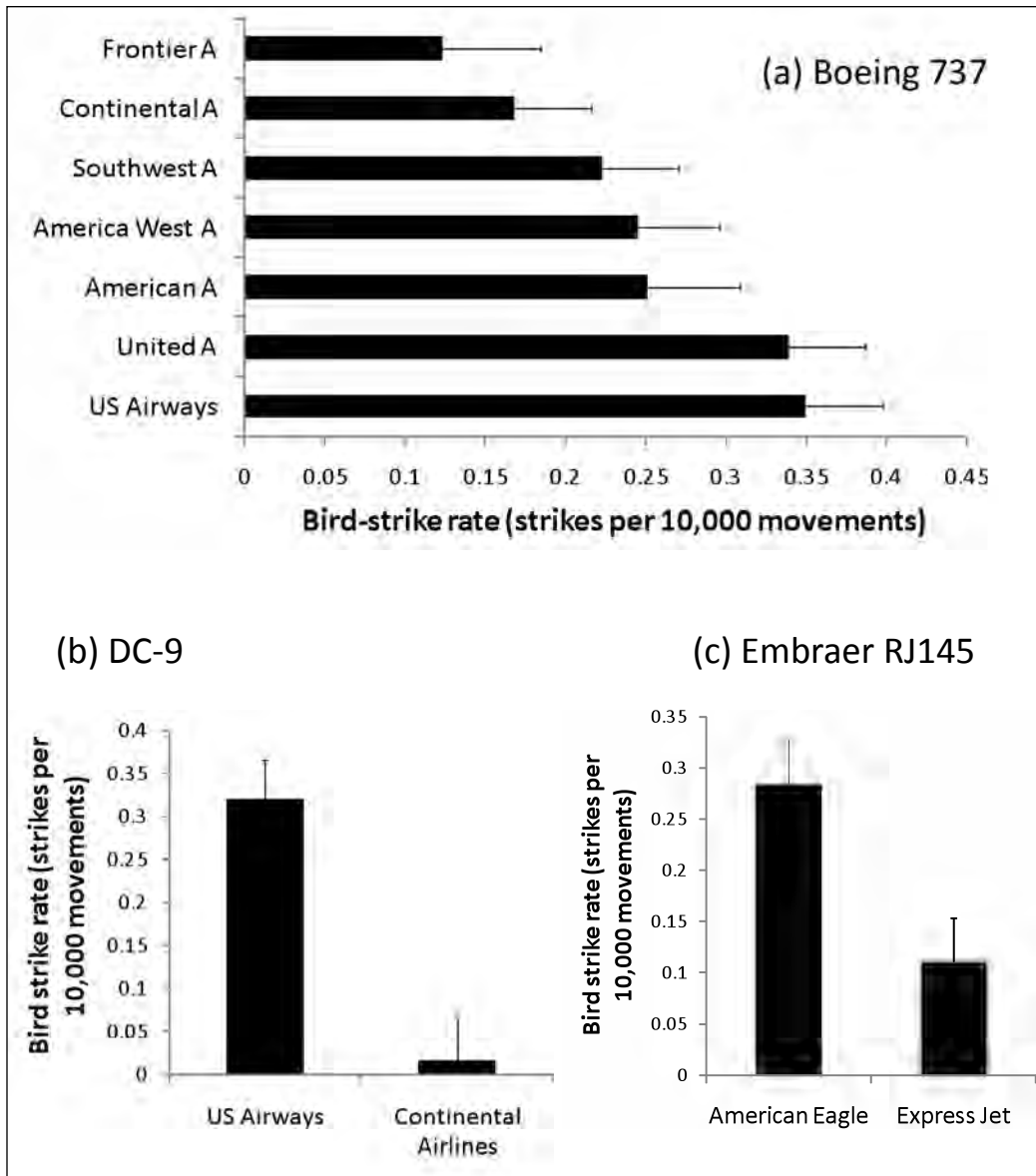
Figure 1. Bird-strike rates estimated as number of bird–aircraft collisions per 10,000 departures or movements in different airlines (a) within 3 different aircraft types: (a) Boeing 737, (b) DC-9, and (c) Embraer RJ145. Shown are \bar{x} \pm SE .
